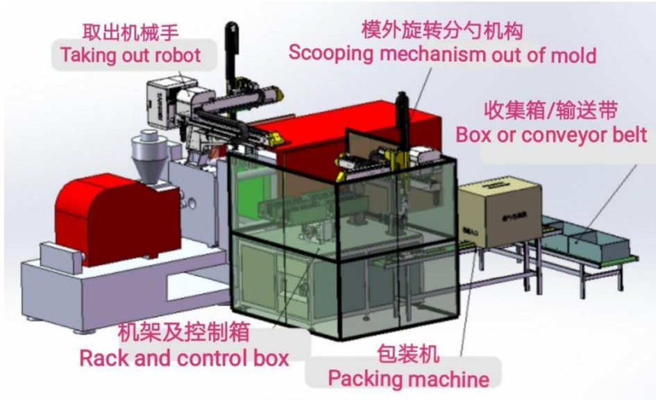
Scooping mechanism
